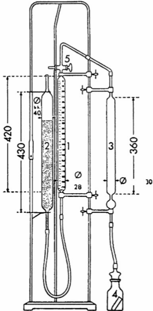
SCHEIBLER-DIETRICH APPARATUS FOR THE DETERMINATION OF CO 2
